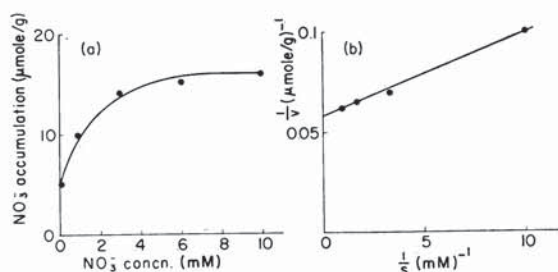
FIG. 6. Dependence of the rate of nitrate accumulation on the concentration of nitrate in the medium for tobacco cells. The nitrate concentration was measured after 10 hr.
