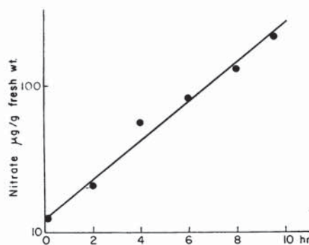
FIG. 5. Nitrate uptake by tobacco cells.
