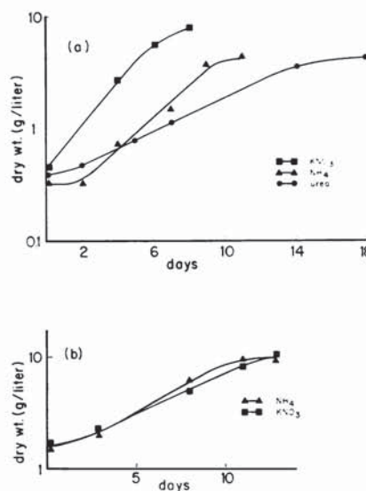
FIG. 1. Growth curves of tobacco and carrot cells on several media. a: Tobacco cells; b: carrot cells.
