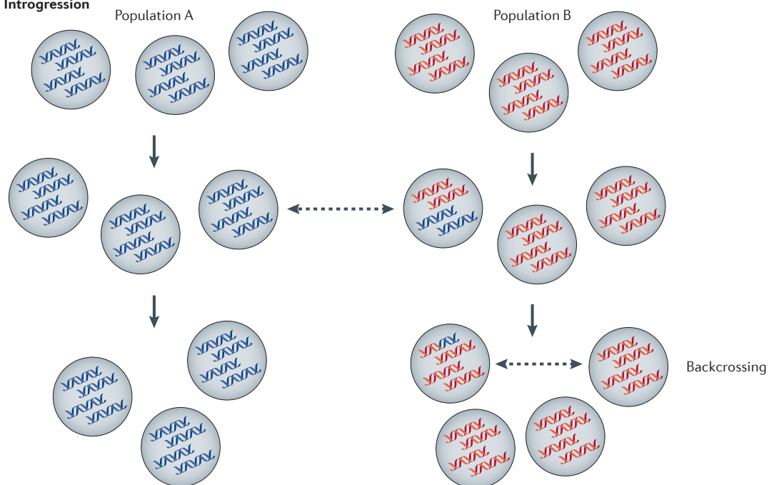
g Introgression
